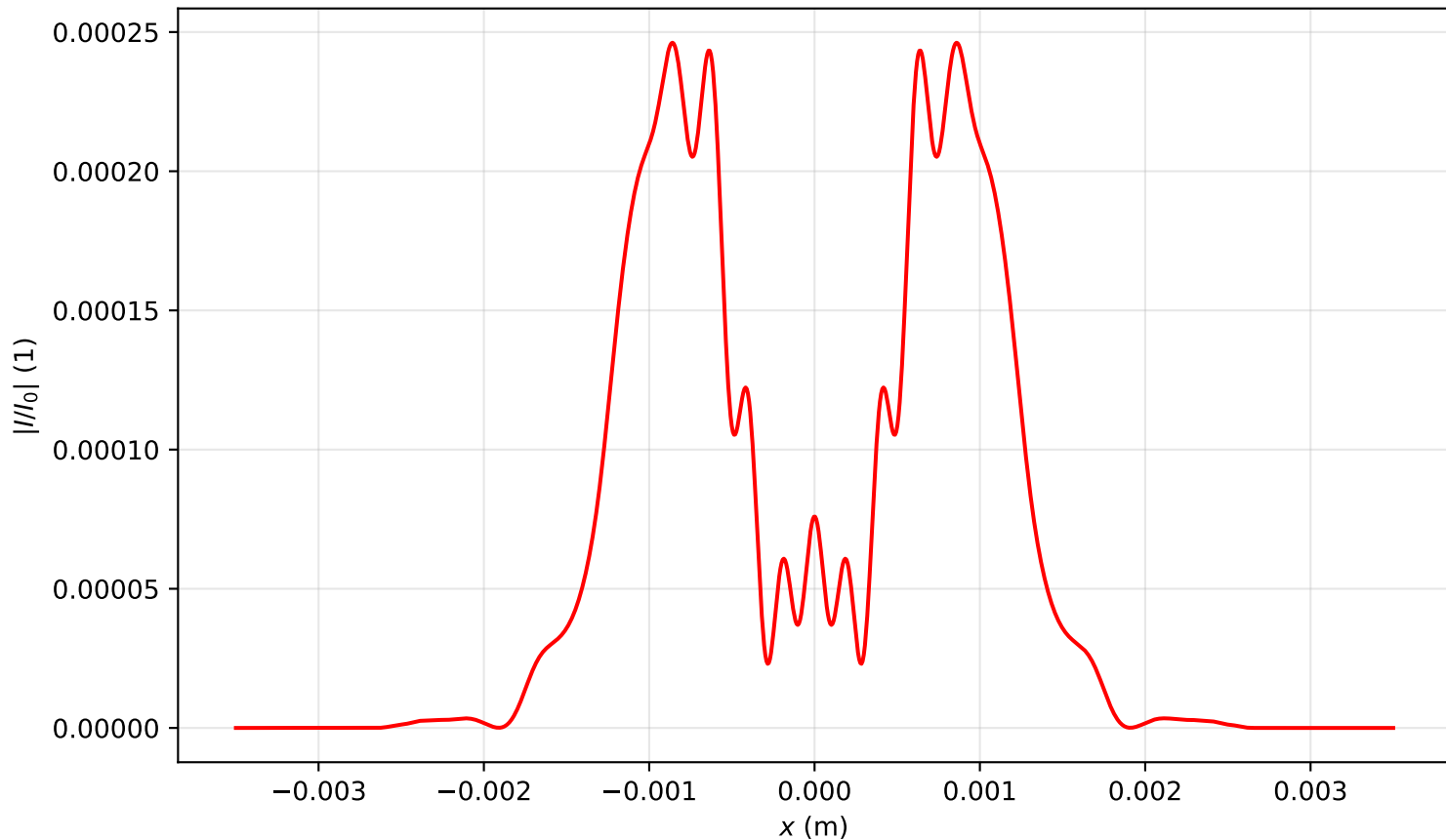
Intensity profile I(x, y = 0, z = 1.115)/I_0 , P_{in}=8.0P_{cr} , artificial time
